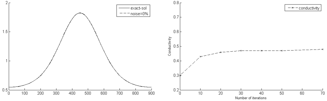
Figure 1: Reconstructed Dirichlet data over \Gamma_i (left) and reconstructed conductivity as a function of iterations (right), where the value of the reconstructed conductivity at convergence is 0.48
